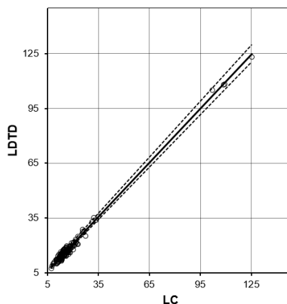
Figure 6 – Passing-Bablok regression curve
